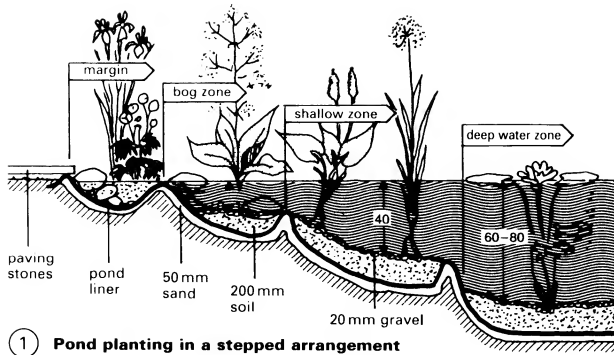
① Pond planting in a stepped arrangement
